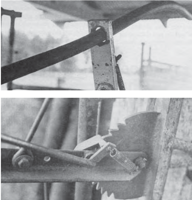
FIGURE 11-3. Latching systems. Steel plate and rod (note worn plate and bent rod) – top; ratchet type – bottom.
